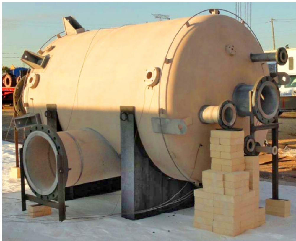
Zirconium kettle rebuilt for MMA/Sulfuric Acid application
